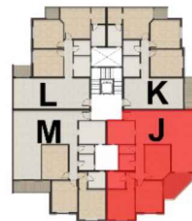
BUILDING 15-18 TYPICAL
